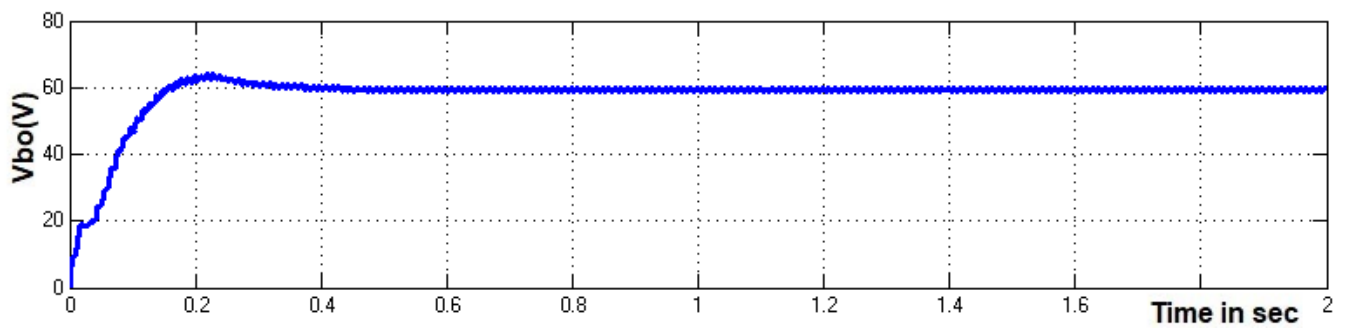
Fig. 11. Voltage across FC boost converter with C-filter.
