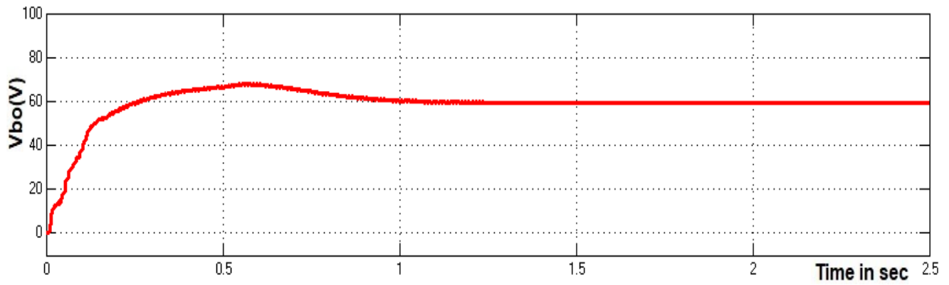
Fig. 39. Flying capacitor voltage in boost converter.
