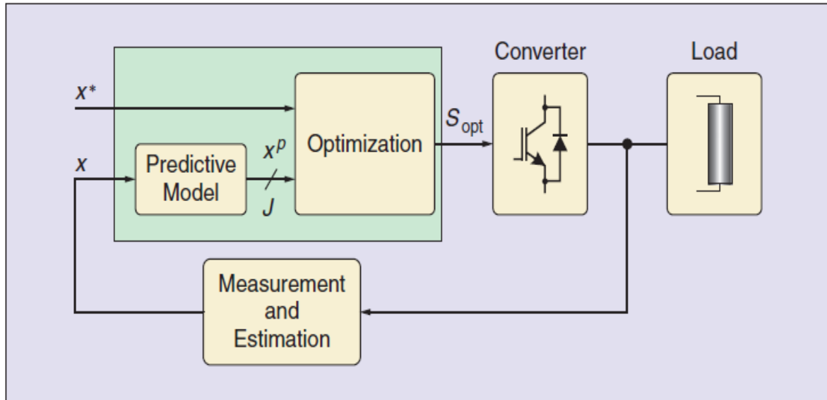
Fig. 5. Block diagram of advanced control with nonlinear gain factors.
