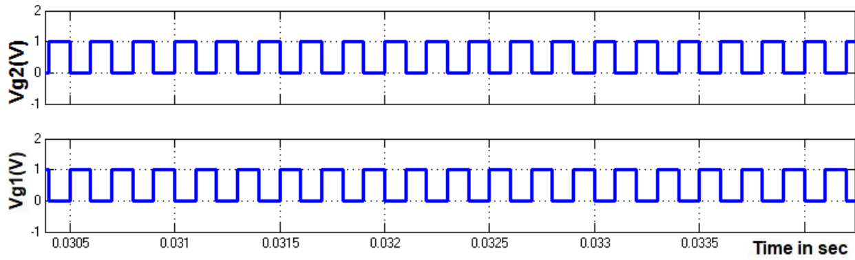
Fig. 18. Complementary pulses for flying capacitor-based DC-DC Converter for the switch S1 and S2
