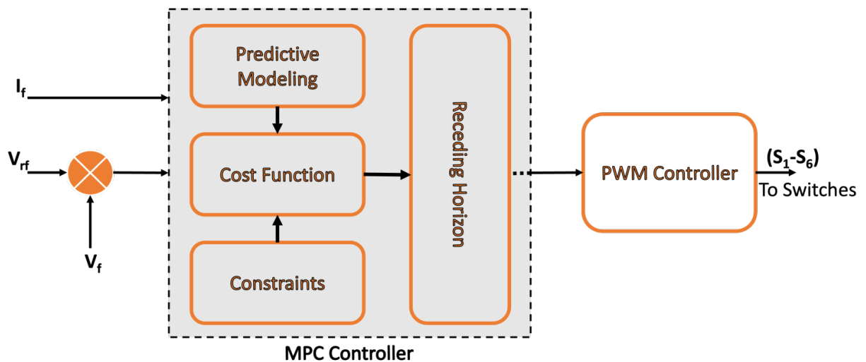
Fig. 37. Schematic of MP control circuit.
