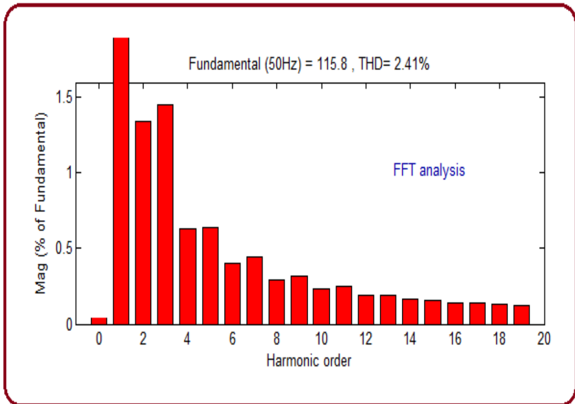
Fig. 33. Voltage harmonics.
