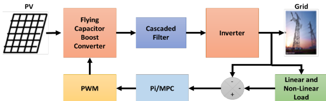
Fig. 3. Proposed closed-loop simulation with model predictive controller.
