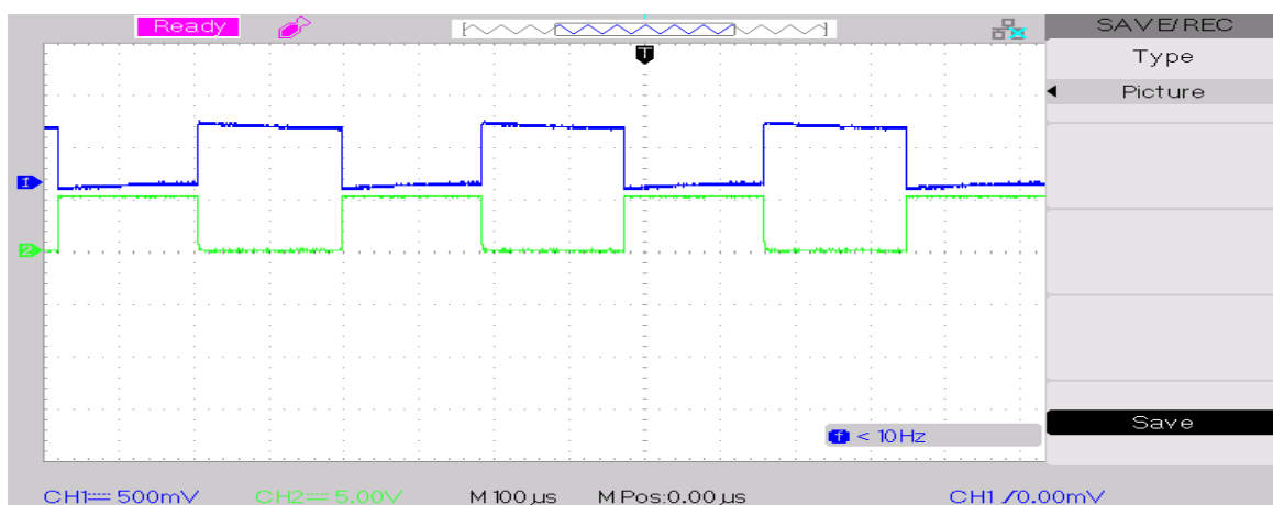
Fig. 49. Switching pulses for inverter of FC-BC.
