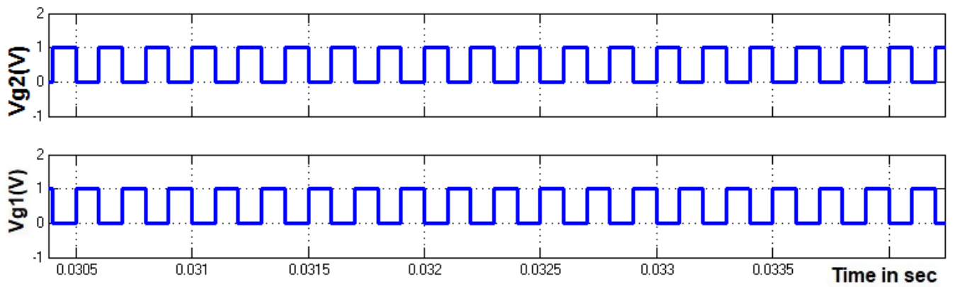
Fig. 10. MOSFET Gate Pulses of FC-boost converter with C-filter.
