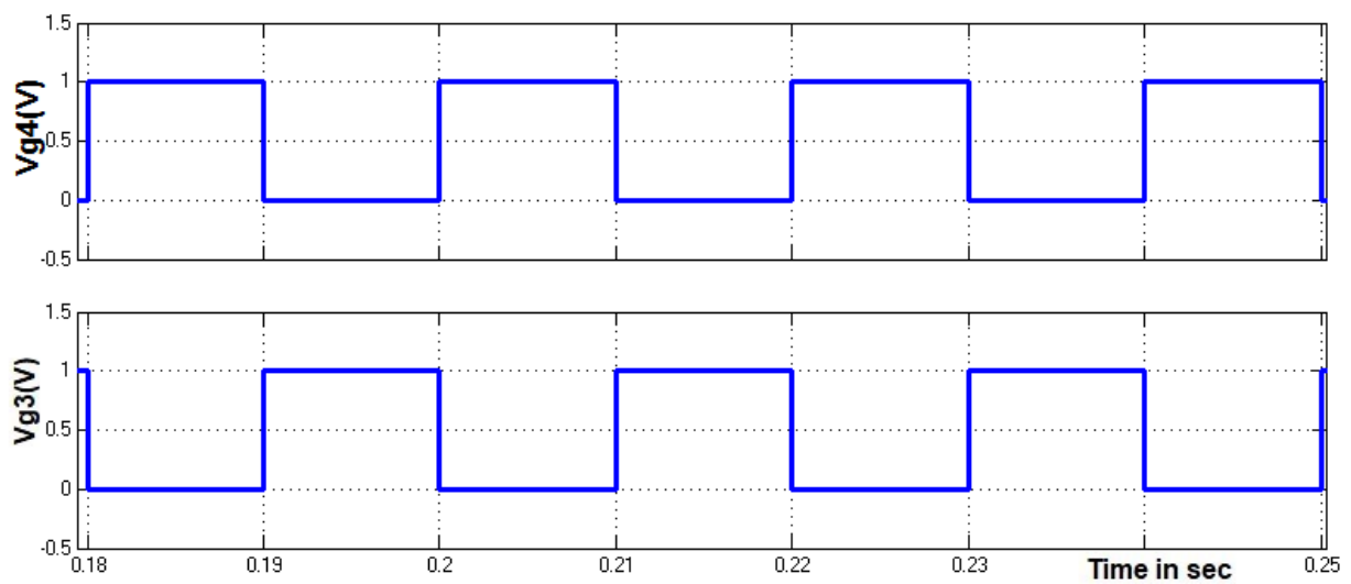
Fig. 22. Complementary pulses for the H-bridge inverter of switch M3 and M4.
