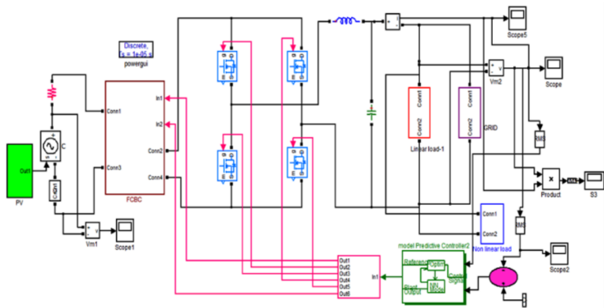
Fig. 36. Closed maximum power controller with grid tie inverter and a flying capacitor-based DC-DC converter.
