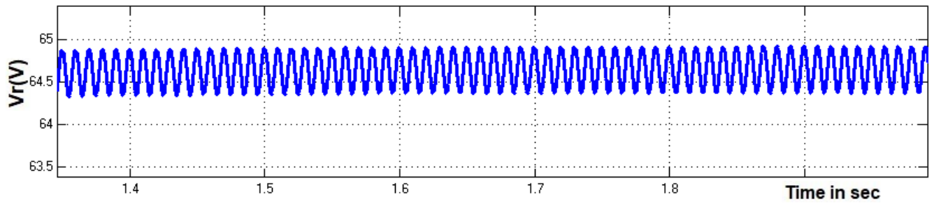
Fig. 21. Ripple Voltage across FC-boost converter with cascaded filter and grid-connected inverter system.
