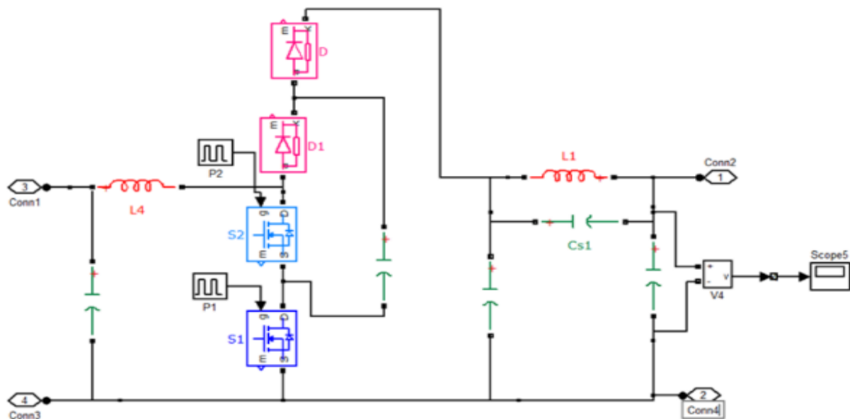
Fig. 19. Half-controlled flying capacitor-based DC-DC converter with series L and cascaded C filters.
