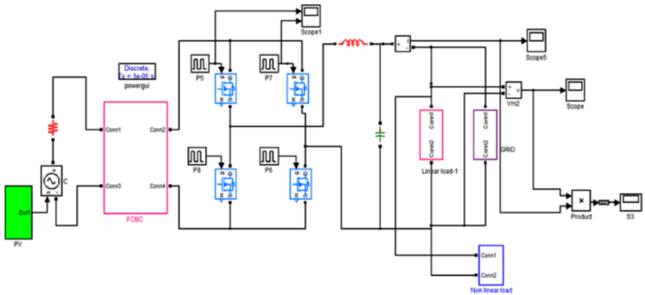
Fig. 16. Flying capacitor-based DC-DC Converter and H bridge inverter grid tie inverter with series L and cascaded C filter.
