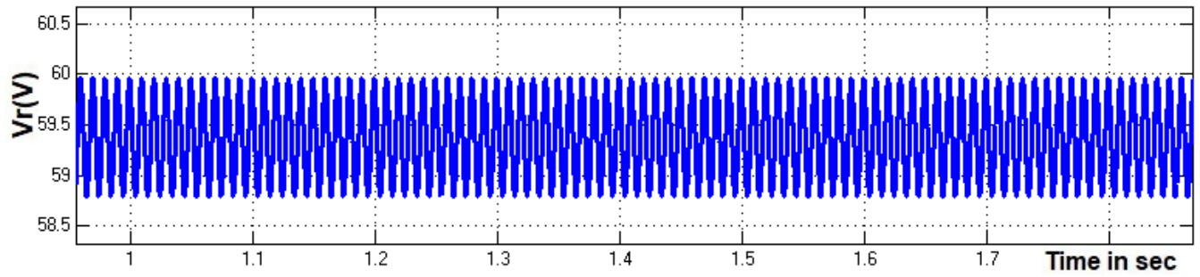
Fig. 12. Ripple voltage across FC boost converter with C-filter and grid-connected inverter system.
