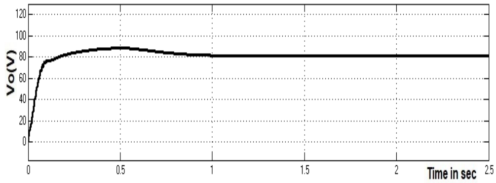
Fig. 42. RL load RMS voltage of flying capacitor-based converter and grid tie inverter with MP controller.
