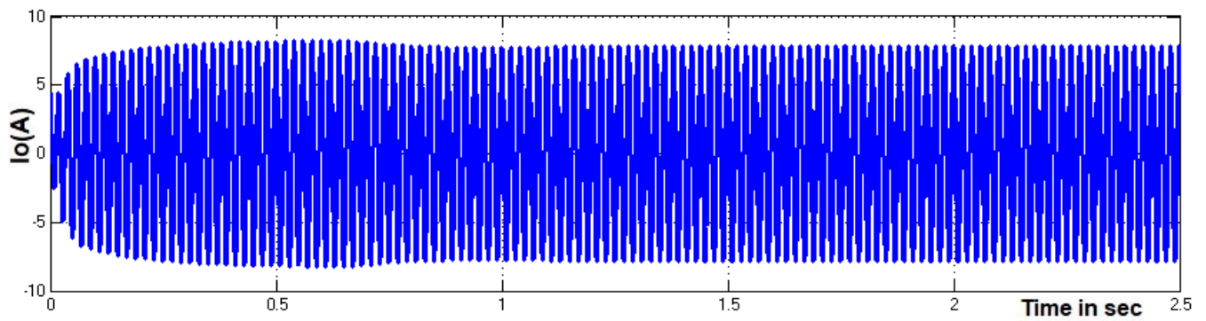
Fig. 41. RL load current of the flying capacitor-based converter and grid tie inverter with MP controller.
