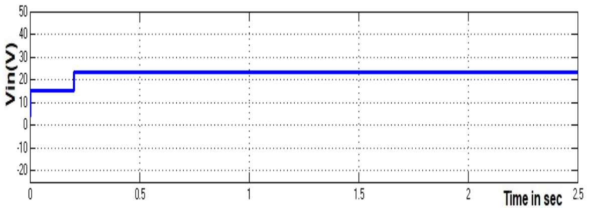
Fig. 28. Input voltage of FC-boost converter with a cascaded filter with closed loop PI controller.
