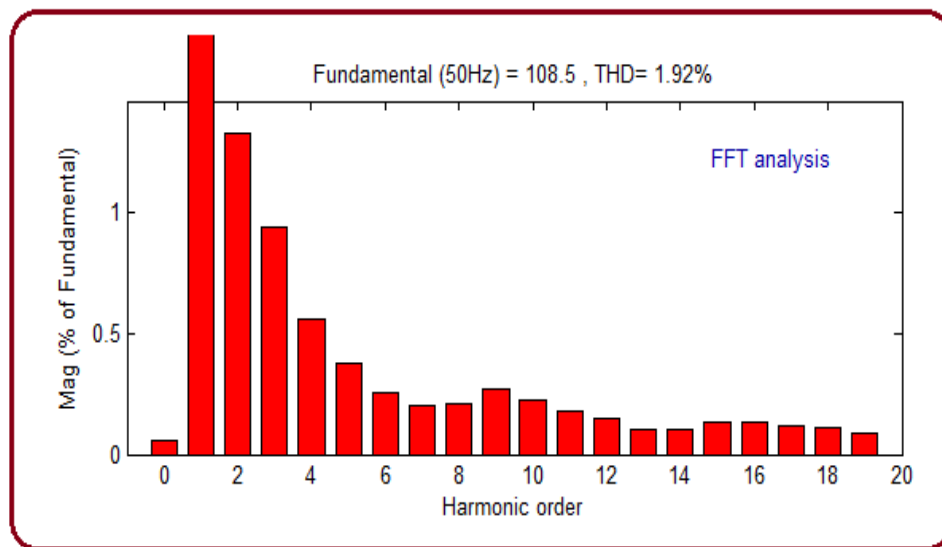
Fig. 43. Voltage harmonics.
