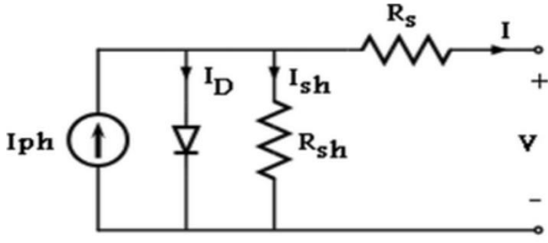
Fig. 6. Photovoltaic cell equivalent circuit.
