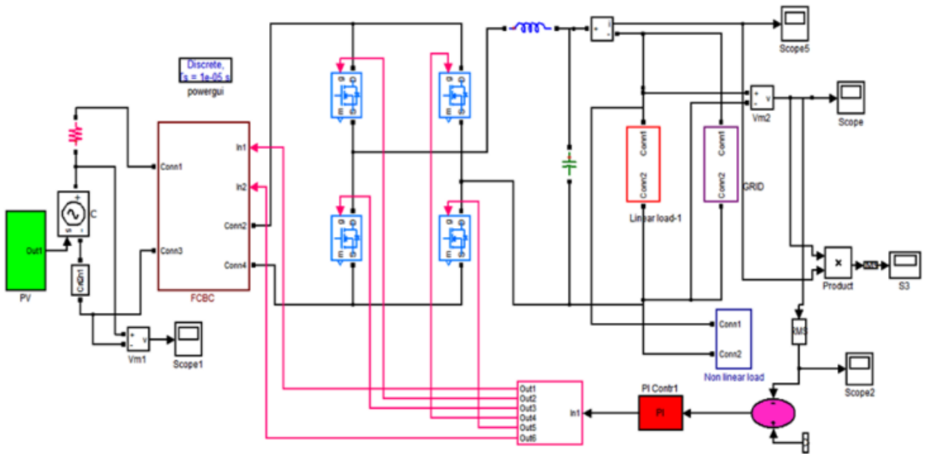
Fig. 27. Closed-loop PI Control for grid tie-inverter and flying capacitor-based DC-DC Converter.
