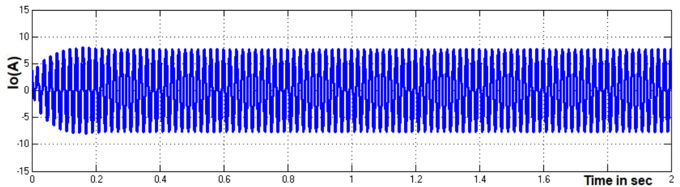
Fig. 13. Current through RL load of FC boost converter with the C-filter and grid tie inverter system.
