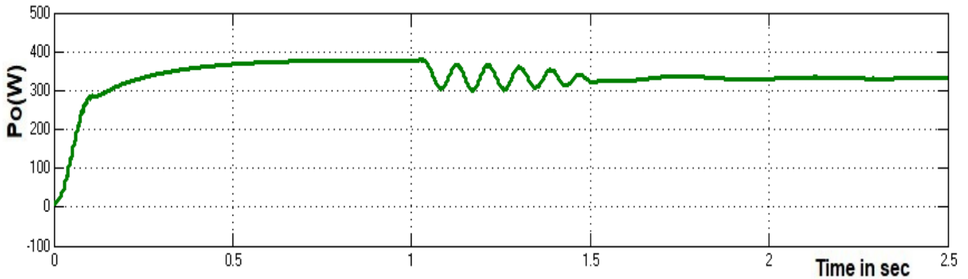
Fig. 35. Output power of FC-boost converter with cascaded filter and grid-connected system with closed loop PI controller.
