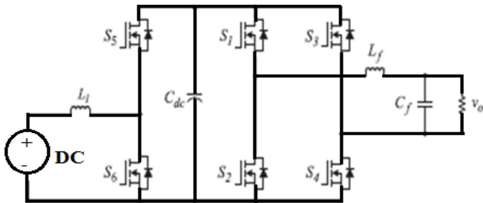
Fig. 2. Existing circuit diagram
