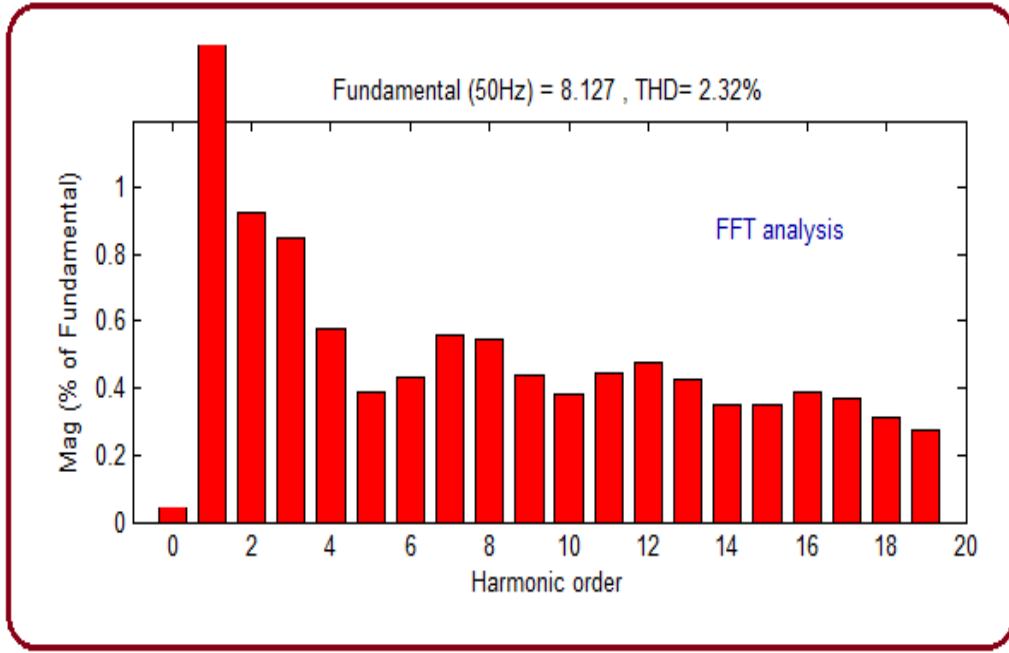
Fig. 34. Current harmonics.
