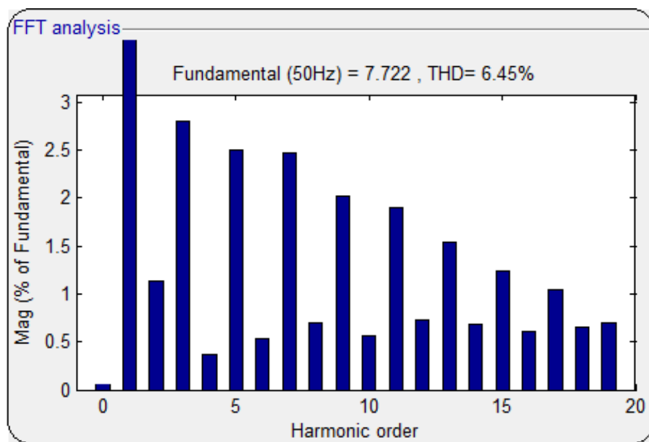
Fig. 14. Current THD of FC-boost converter with C-filter.
