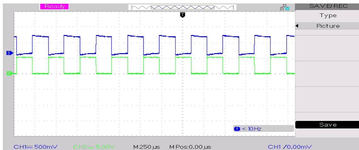
Fig. 48. Switching pulse of FC-BC.
