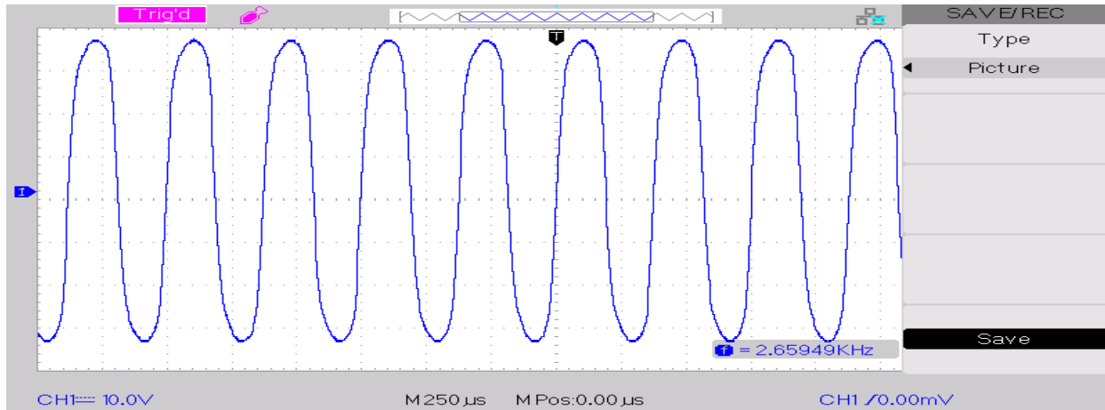
Fig. 51. Voltage across the inverter terminals of FC-BC.
