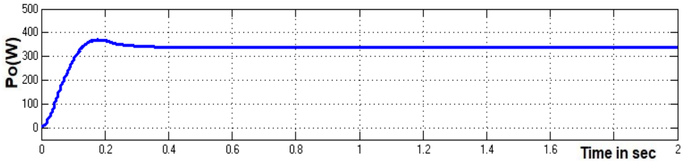
Fig. 15. Output power of FC-boost converter with C-filter and grid-connected inverter system
