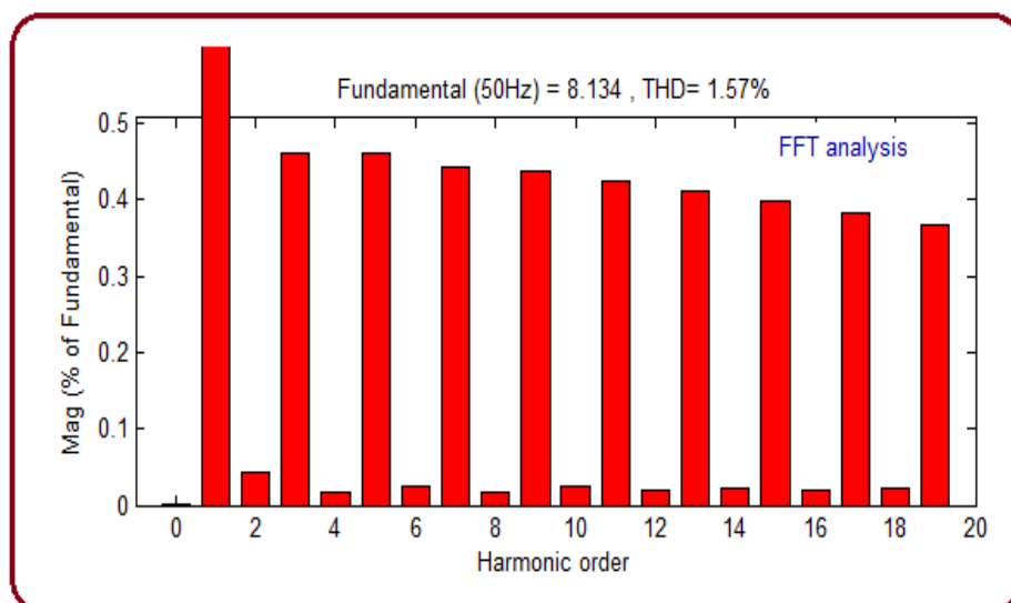
Fig. 44. Current harmonics.
