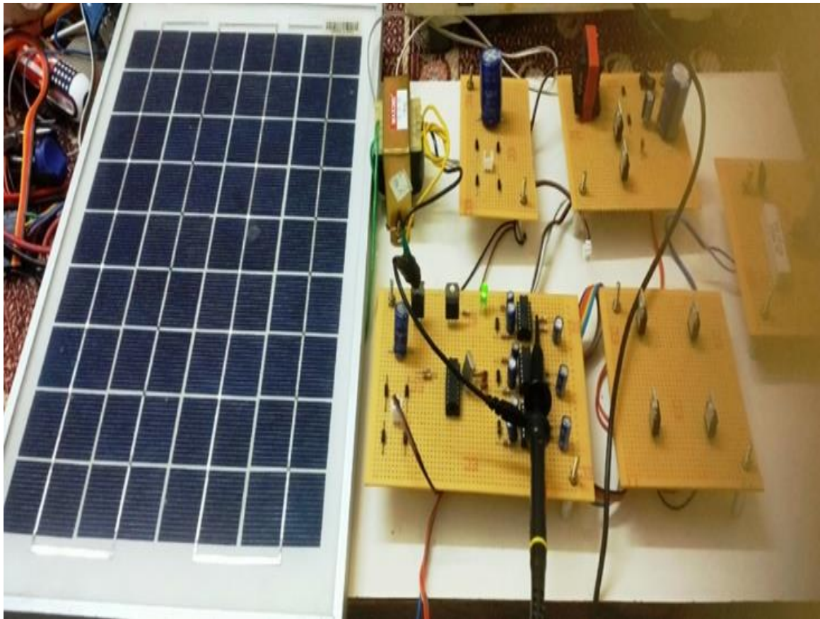
Fig. 46. Hardware snapshot of FC-BC and grid-connected inverter system.
