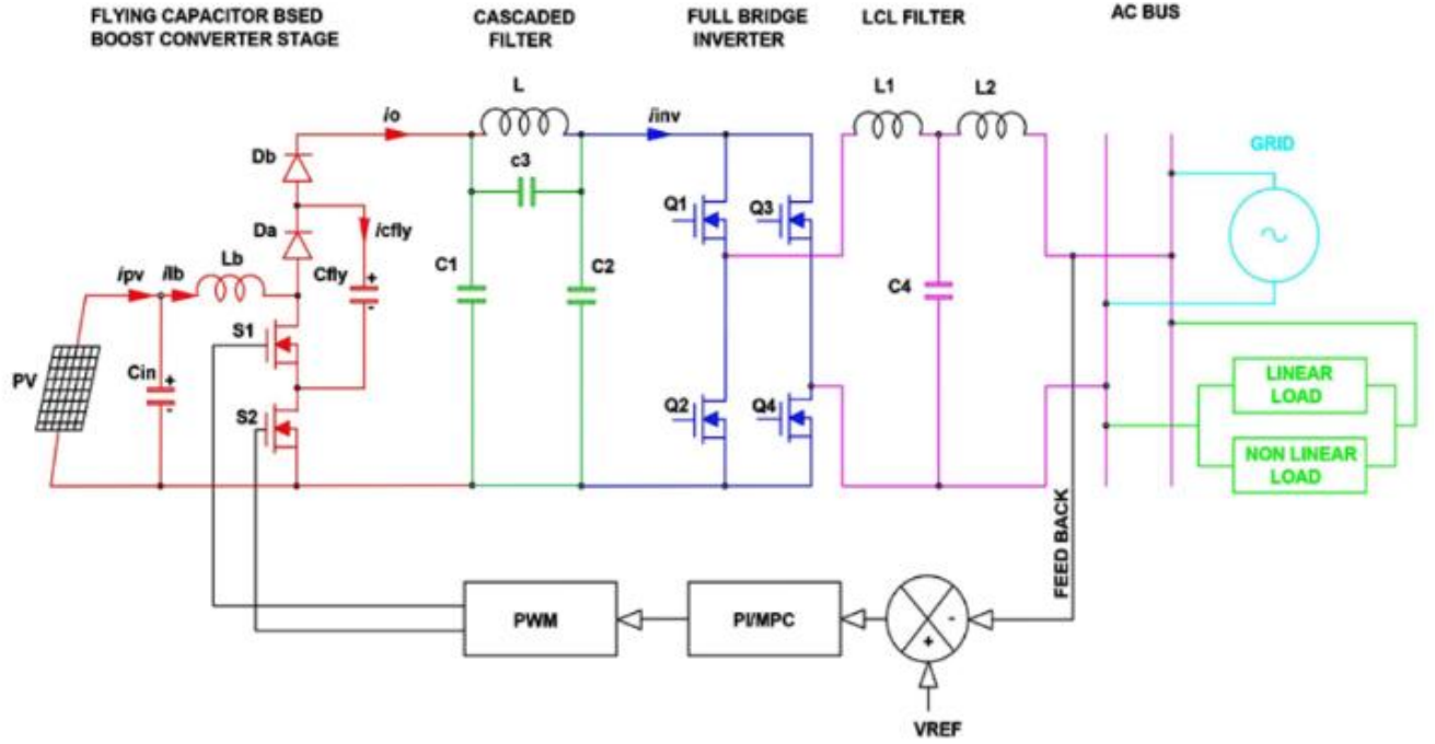
Fig. 4. Circuit diagram of a closed-loop-controlled PV grid-connected system.
