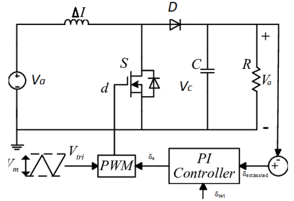
Fig. 7. Boost converter in closed-loop operation.
