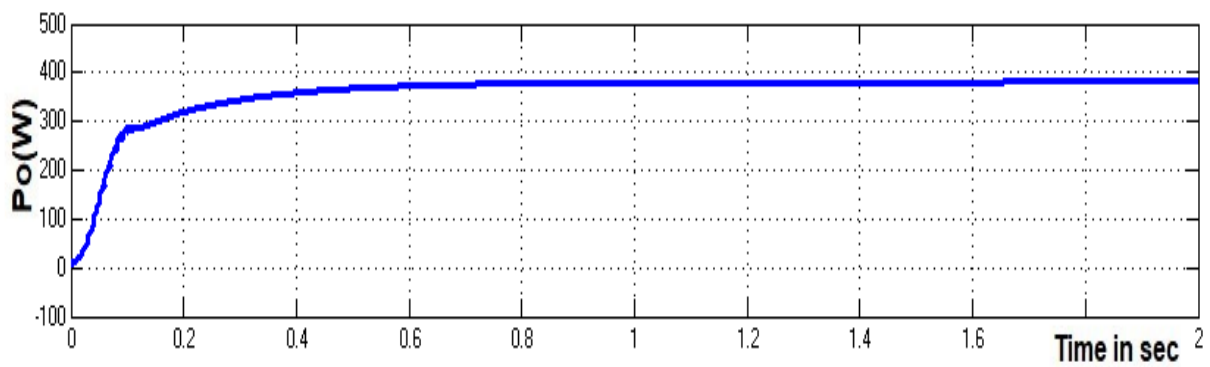
Fig. 26. Grid tie-inverter with FC-based boost converter power output.
