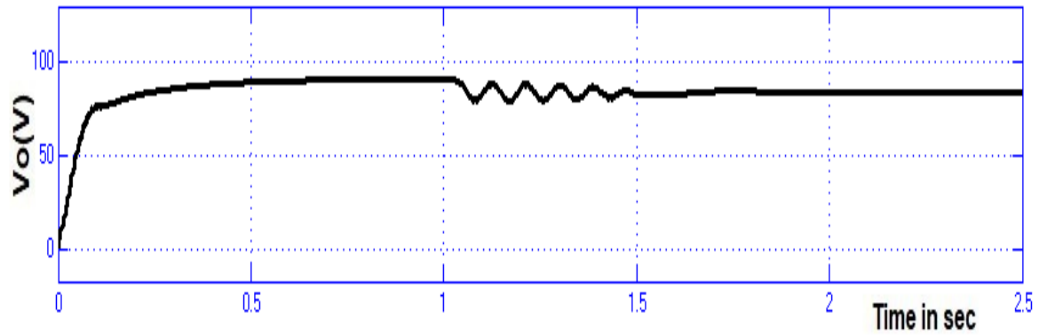
Fig. 32. RL load RMS voltage.
