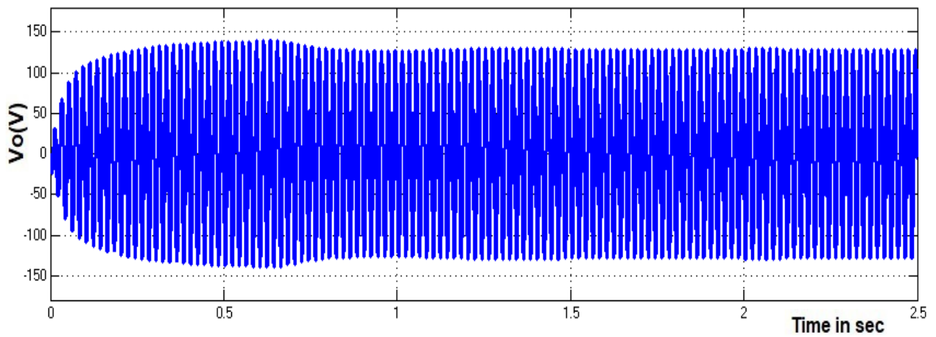
Fig. 40. RL load voltage of DC-DC converter and grid tie inverter system with MP controller.
