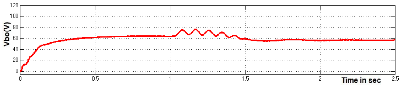
Fig. 29. Flying capacitor voltage in DC-DC Converter.
