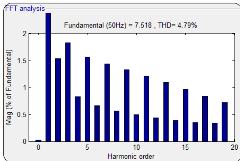
Fig. 25. Current THD of FC-boost converter with cascaded filter and grid-connected inverter system.
