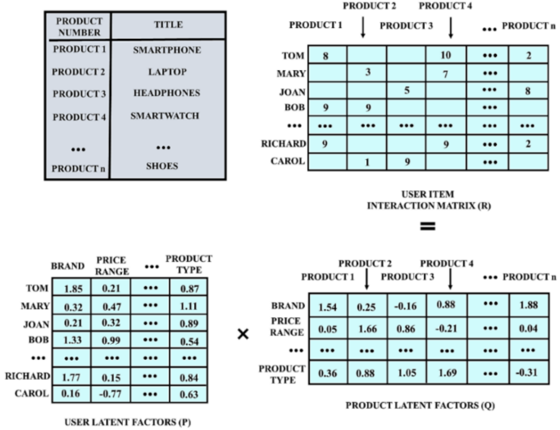
Fig. 4. Decomposing user-product interactions with Latent Factors.
