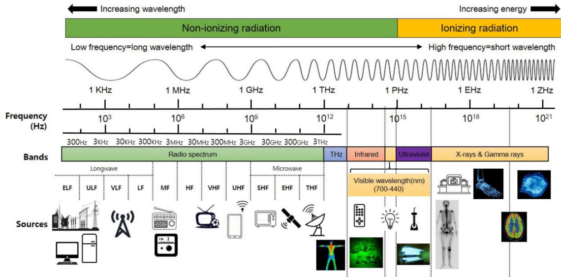
Fig. 1. Diagram showing the range of electromagnetic fields present in our surroundings. [10].
