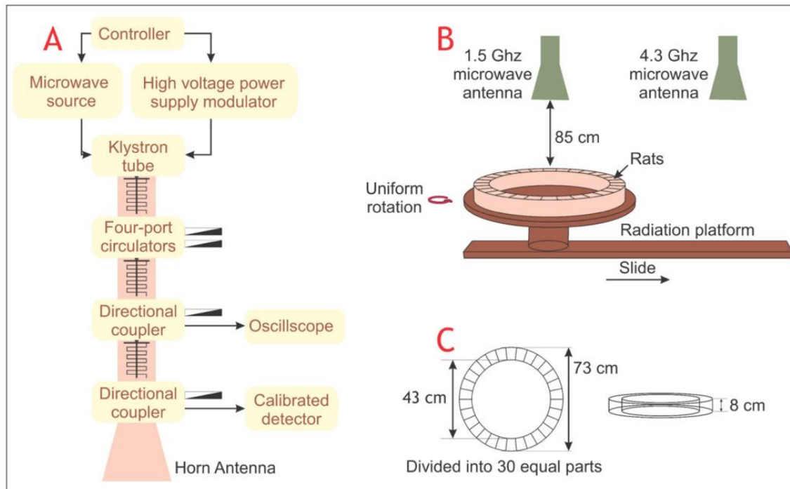
Fig. 2. The experimental setup for RF-EMR exposure includes a microwave source (A), radiation process (B), and a rat container (C). [12].
