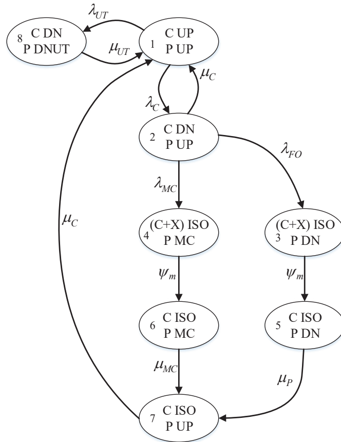
Fig. 2. The proposed Markov model
