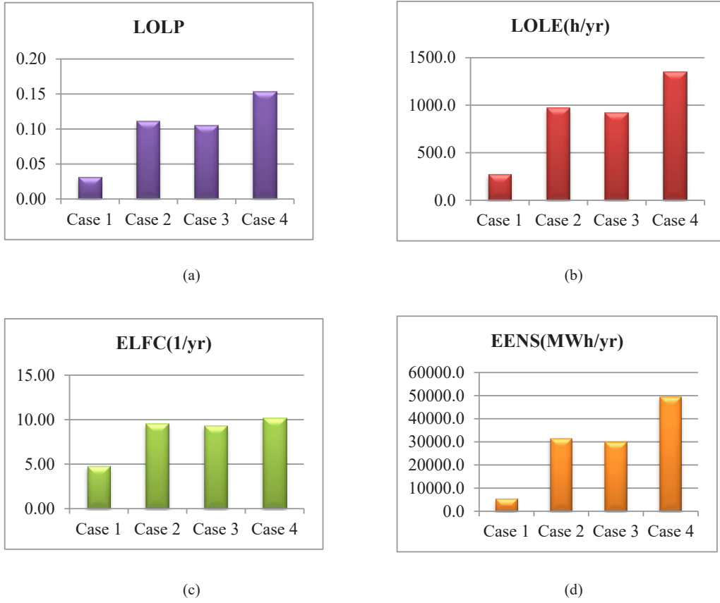
Fig. 10. The reliability indices of LOLP(a), LOLE(b), ELFC(c), and EENS(d) for all 4 cases
