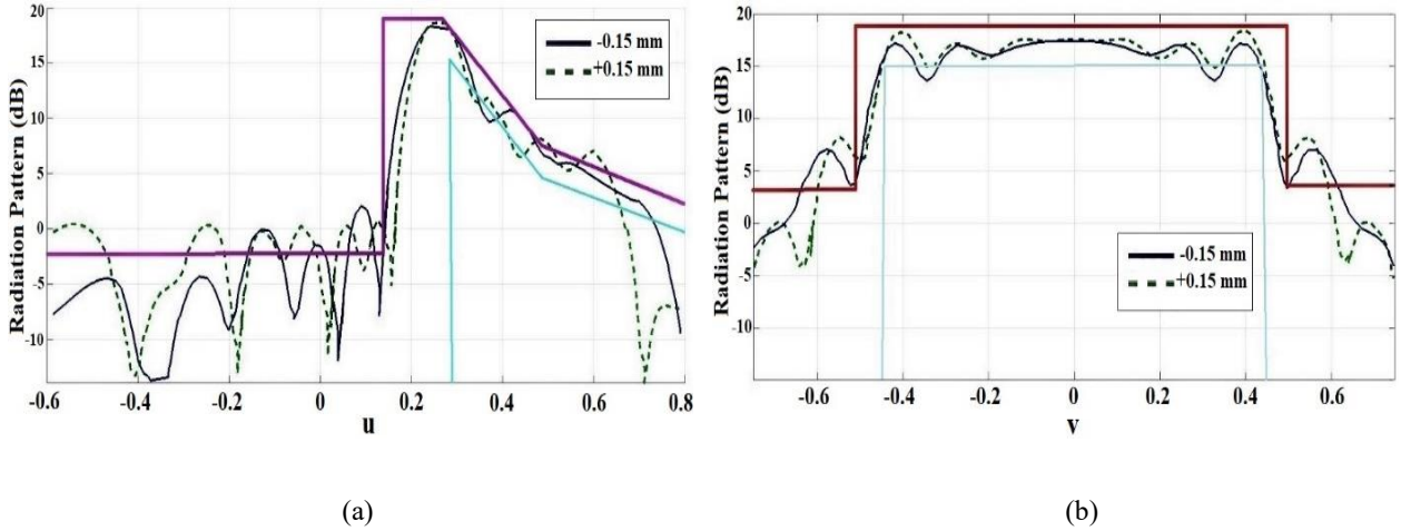
Fig. 3. Radiation patterns of the RA with ±0.15mm tolerance at a) \varphi=0^\circ plane, b) \varphi=90^\circ plane
