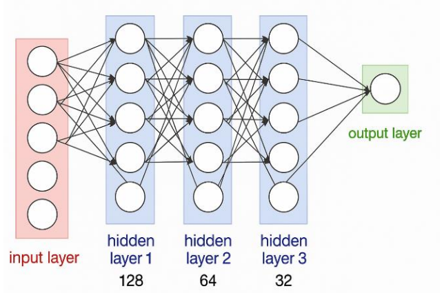
Fig. 4. Shows the main structure of DNN model in the paper.
