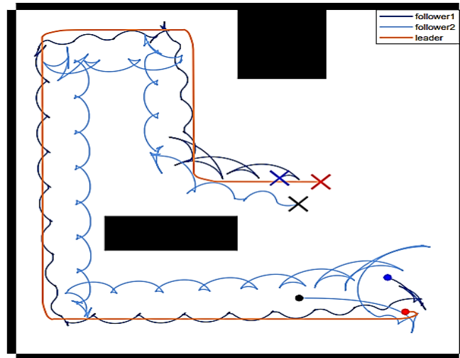
Fig. 13. Simulation of mobile robot's trajectory in a virtual environment with disturbance for followers with PID controller
