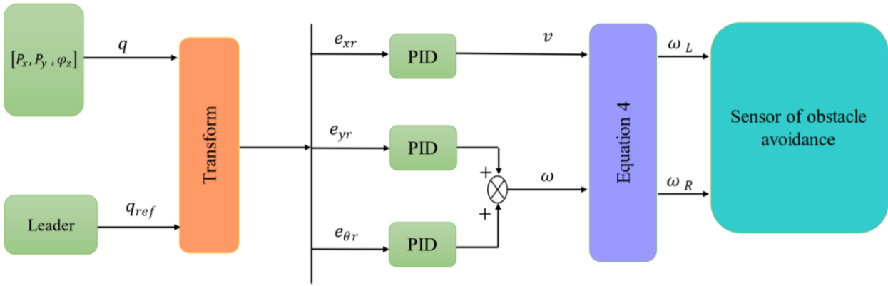
Fig. 2. The complete architecture of the PID-Controller for Mobile Robot
