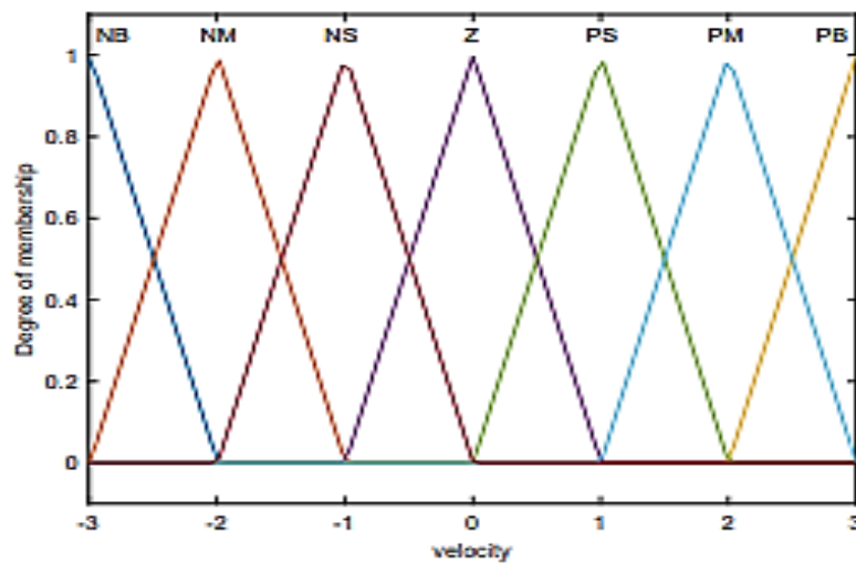
Fig. 5. Output membership function for velocity
