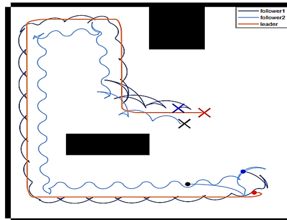
Fig. 15. Simulation of mobile robot's trajectory in a virtual environment with disturbance for followers with fuzzy controller
