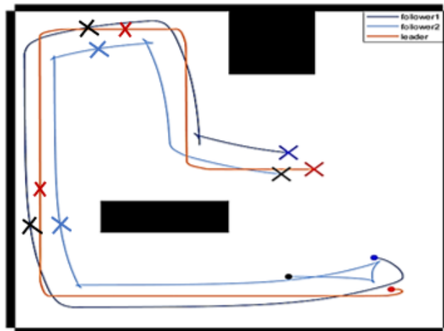
Fig. 11. Simulation of mobile robot's trajectory in a virtual environment without disturbance for followers with fuzzy controller
