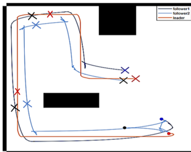
Fig. 9. Simulation of mobile robots' trajectory in a virtual environment without disturbance for followers with PID controller
