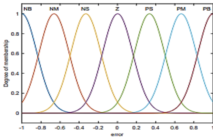
Fig. 4. Input membership for error and error change
