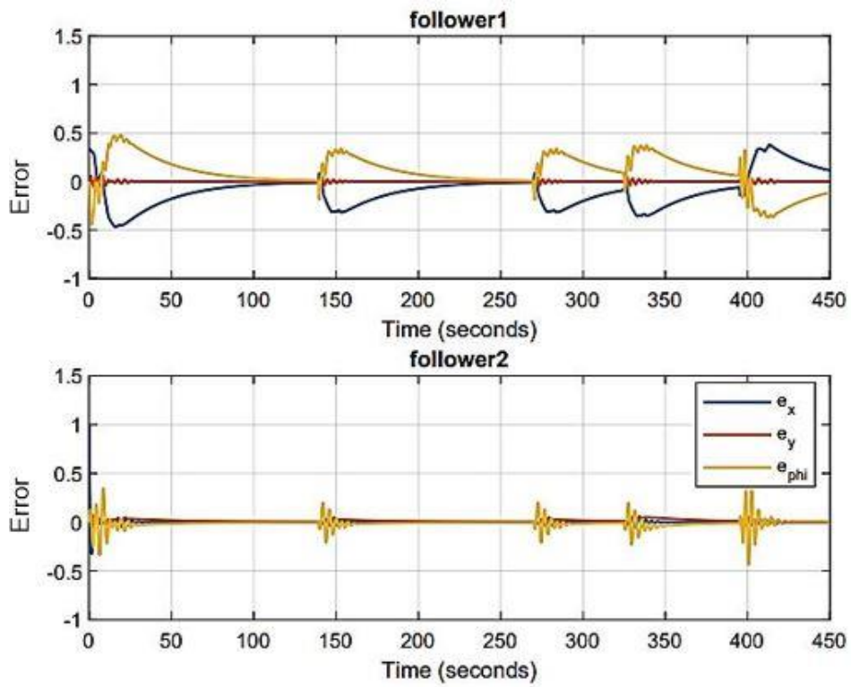
Fig. 8. Position and orientation errors for follower mobile robots with PID without disturbance
