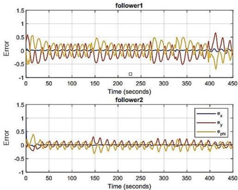
Fig. 14. Position and orientation errors for follower mobile robots with FLC
