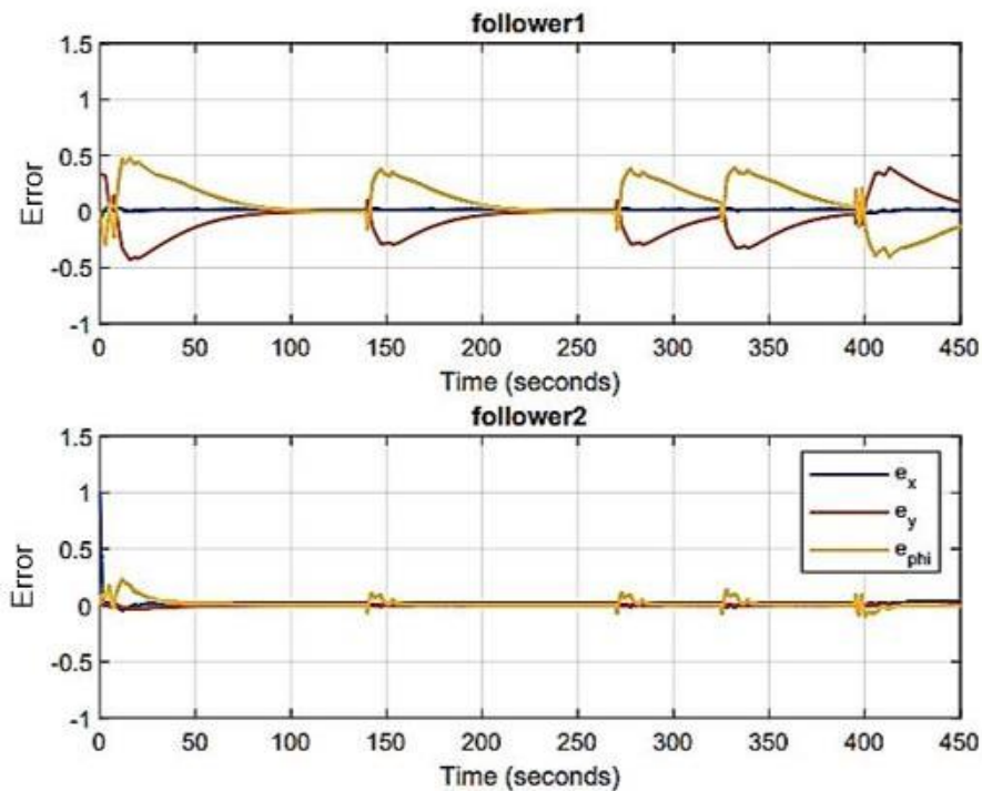
Fig. 10. Position and orientation errors for follower mobile robots with FLC without disturbance
