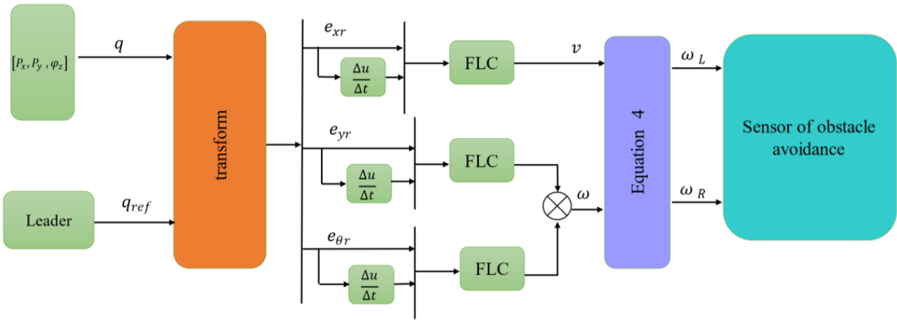
Fig. 3. Complete architecture of the Fuzzy-Controller for Mobile-Robot
