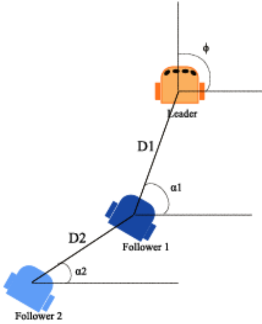
Fig. 6. Mobile robot model and leader-following formation[19]
