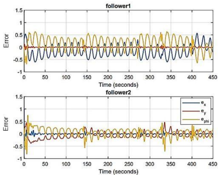
Fig. 12. Position and orientation errors for follower mobile robots with PID with disturbance
