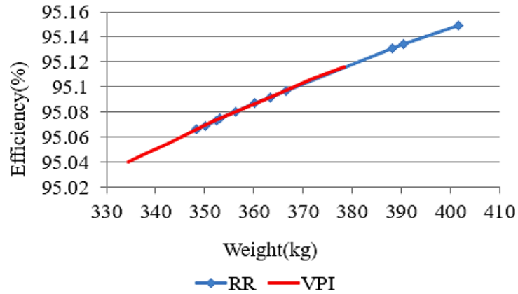
Fig. 14. Sensitivity Efficiency-weight.
