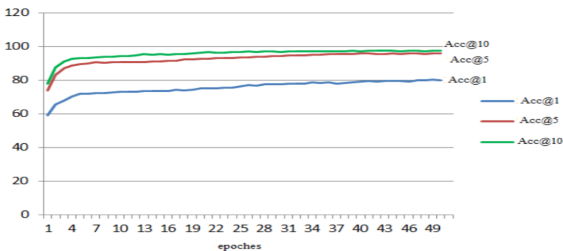
Fig. 3. Accuracy Graph
